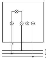
theLeda P12, theLeda P24 (Manual operation via circuit breaker button)
