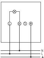
theLeda P12, theLeda P24 (Standard operation)
