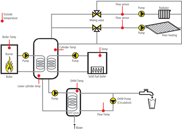
RAMSES 856 top2 OT (in combination with OT-Box 9070712)
