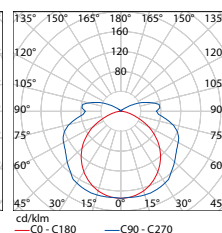
DUST EVG EB PC 2 × 36W
