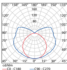
DUST EVG PC 1 ×18W
