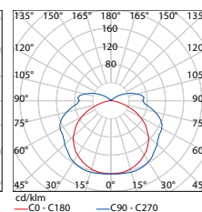
TRUST EVG PC 2 ×58W
