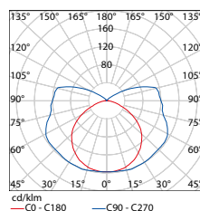
DUST EVG EB PC 1 × 36W
