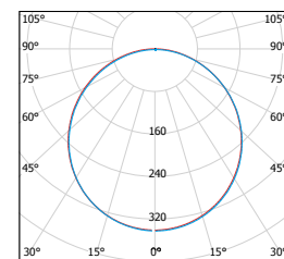
LED VEGA SQUARE
