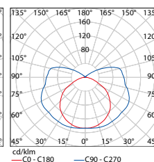
DUST EVG EB PC 1 × 58W
