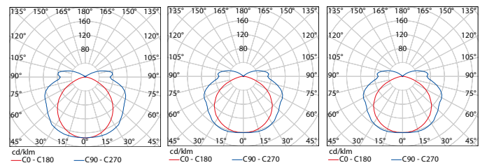
TRUST EVG PS 2 × 18W
