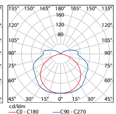
DUST EVG EB PC 2 × 58W
