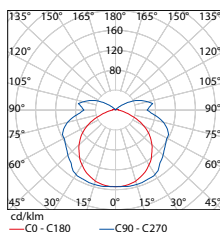
DUST EVG PC 2 ×18W
