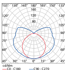
DUST EVG EB PC 1 × 18W
